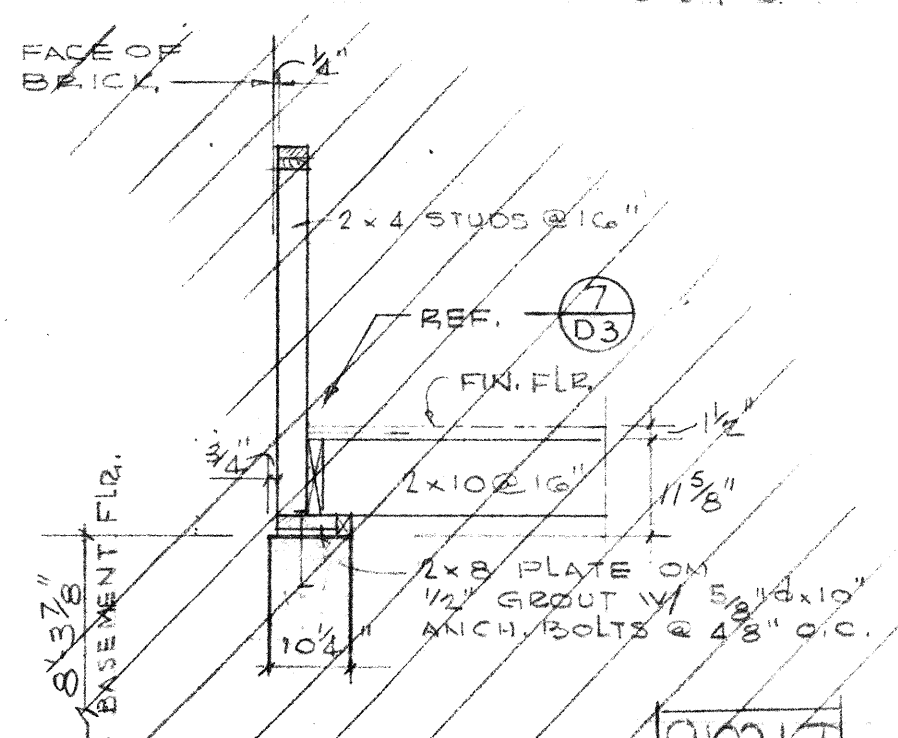
SECTION 1/2" = 1'-0"
