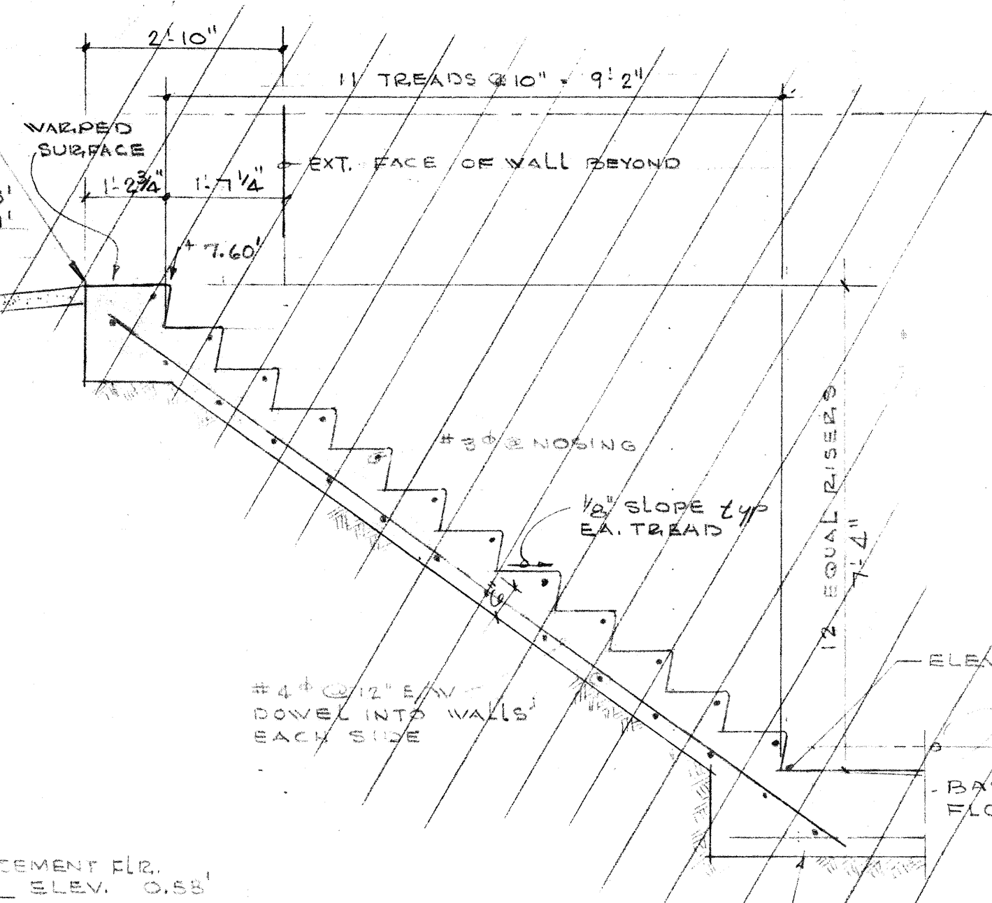
OMIT STAIR SECTION 1/2" = 1'-0"
