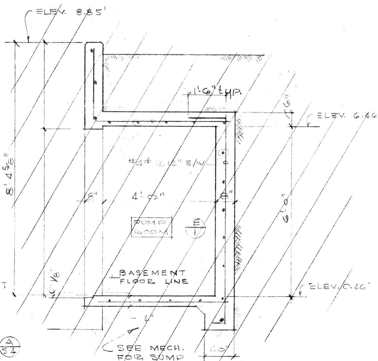
OMIT SECTION 1/2" = 1'-0"
